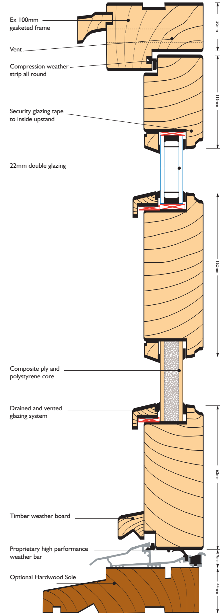
Vertical Section - 'Orkney' style open in door
