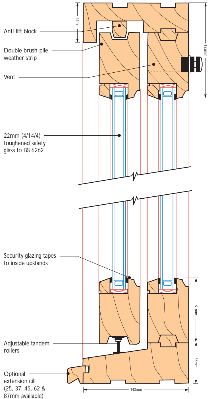
Vertical Section Sliding Patio Doors
