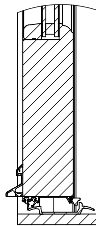
DETAIL G SCALE 1 : 3
