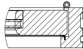
DETAIL G SCALE 1 : 3
